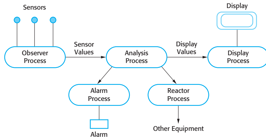
Figure 20.7 Observe and React process structure
