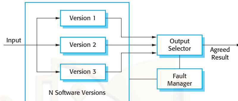
Figure 13.7 N-version programming
